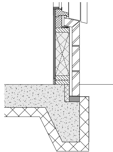
DETAIL 10
