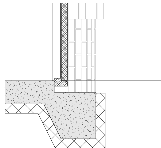
DETAIL 10
