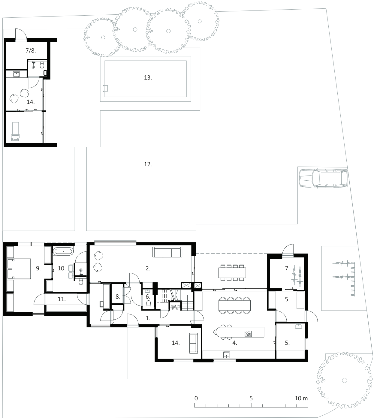
begane grond 2025 | 1:200
