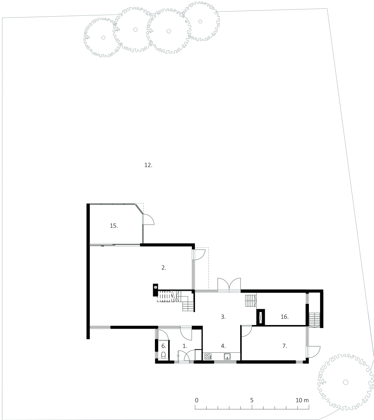
begane grond 1968 | 1:200
