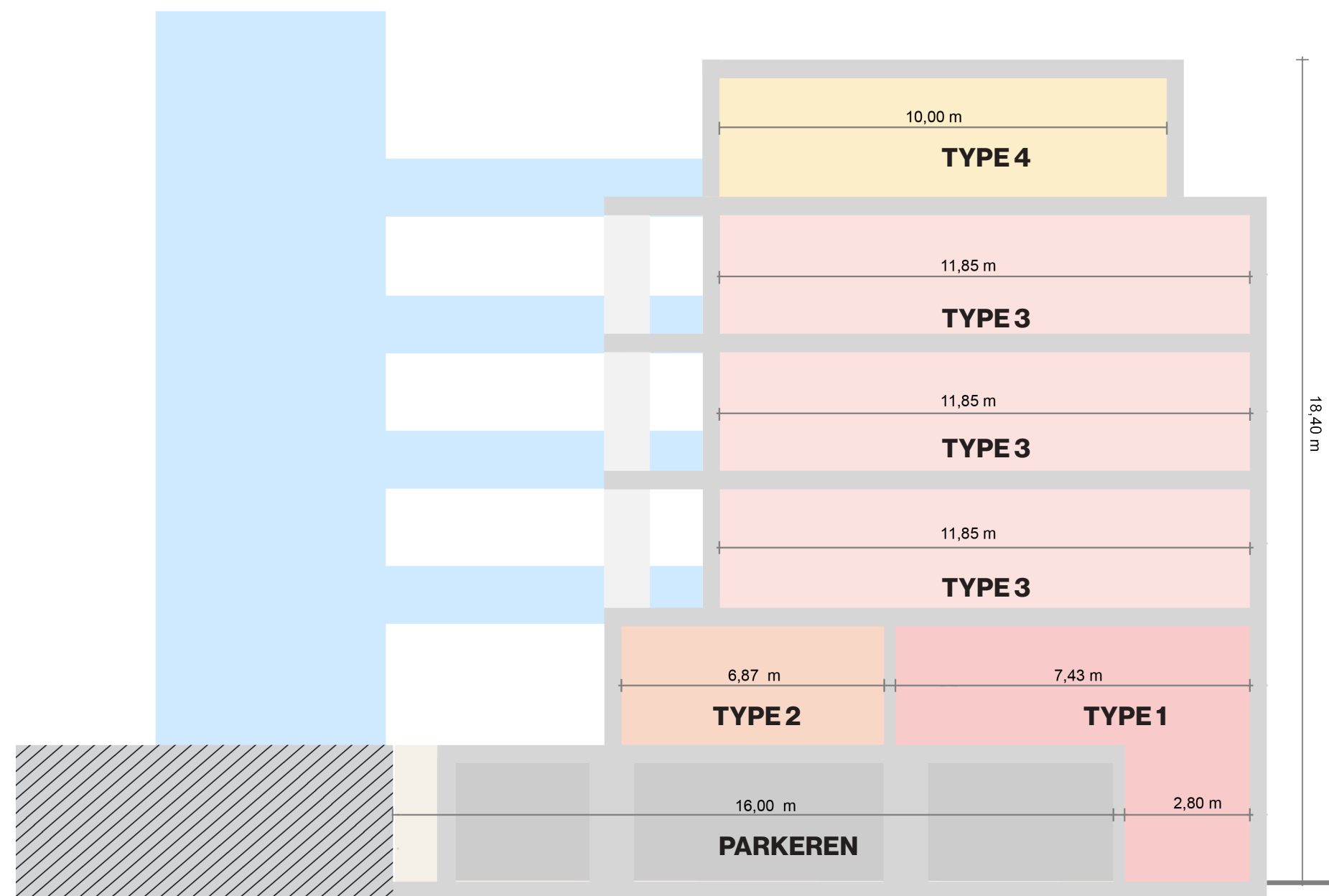
STAPELING VAN VERSCHILLENDE WOONINGTYPES STACKING OF DIFFERENT HOUSING TYPES
