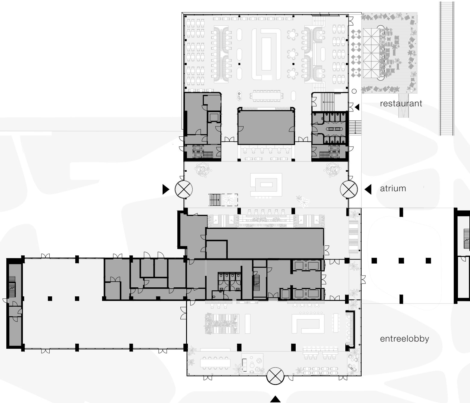
Rembrandt Park One Begane grond | casco plattegrond
