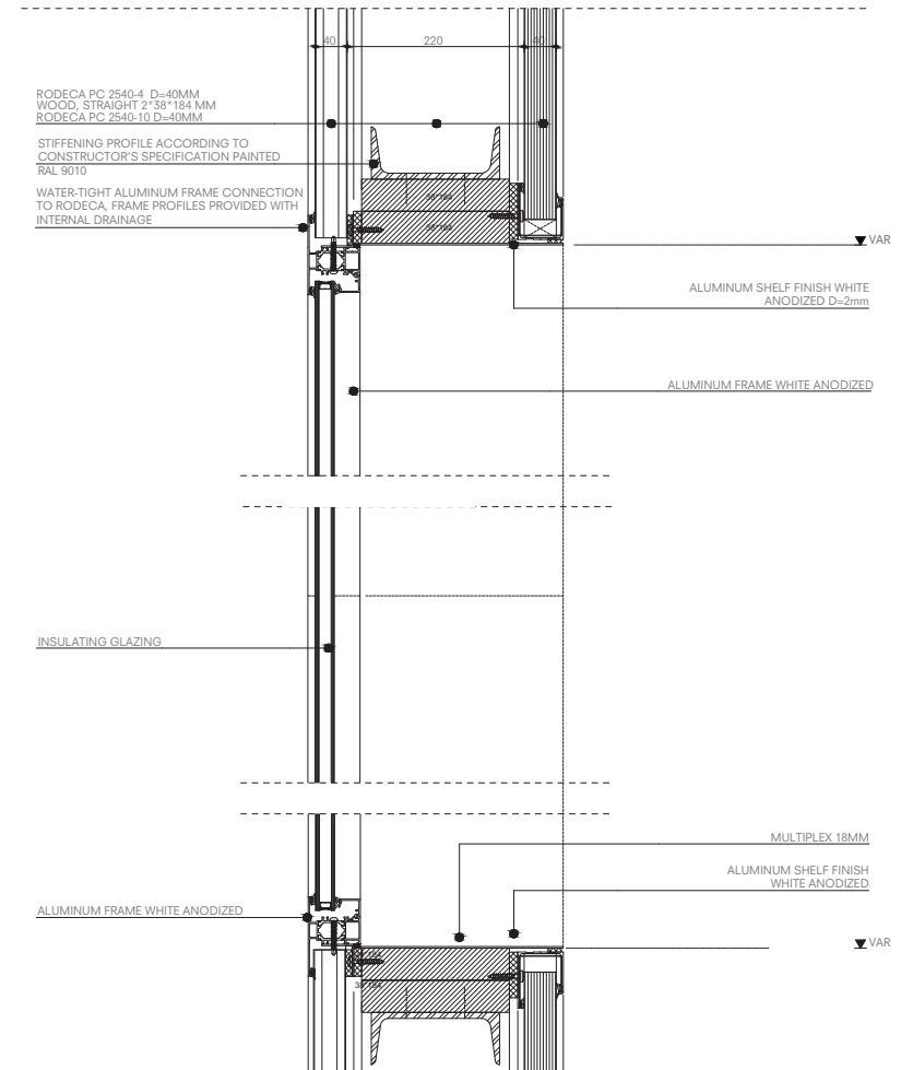
Detail 2: South-West Window
