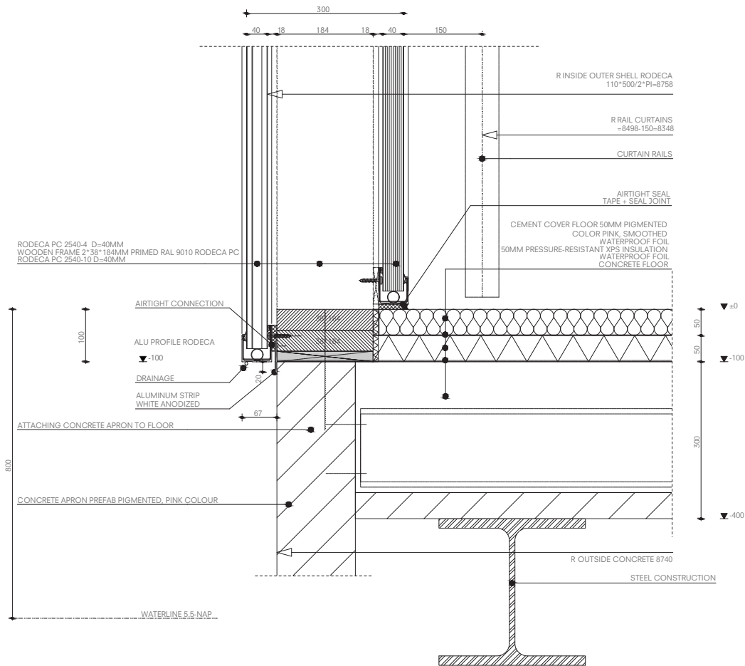
Detail 3: Facade
