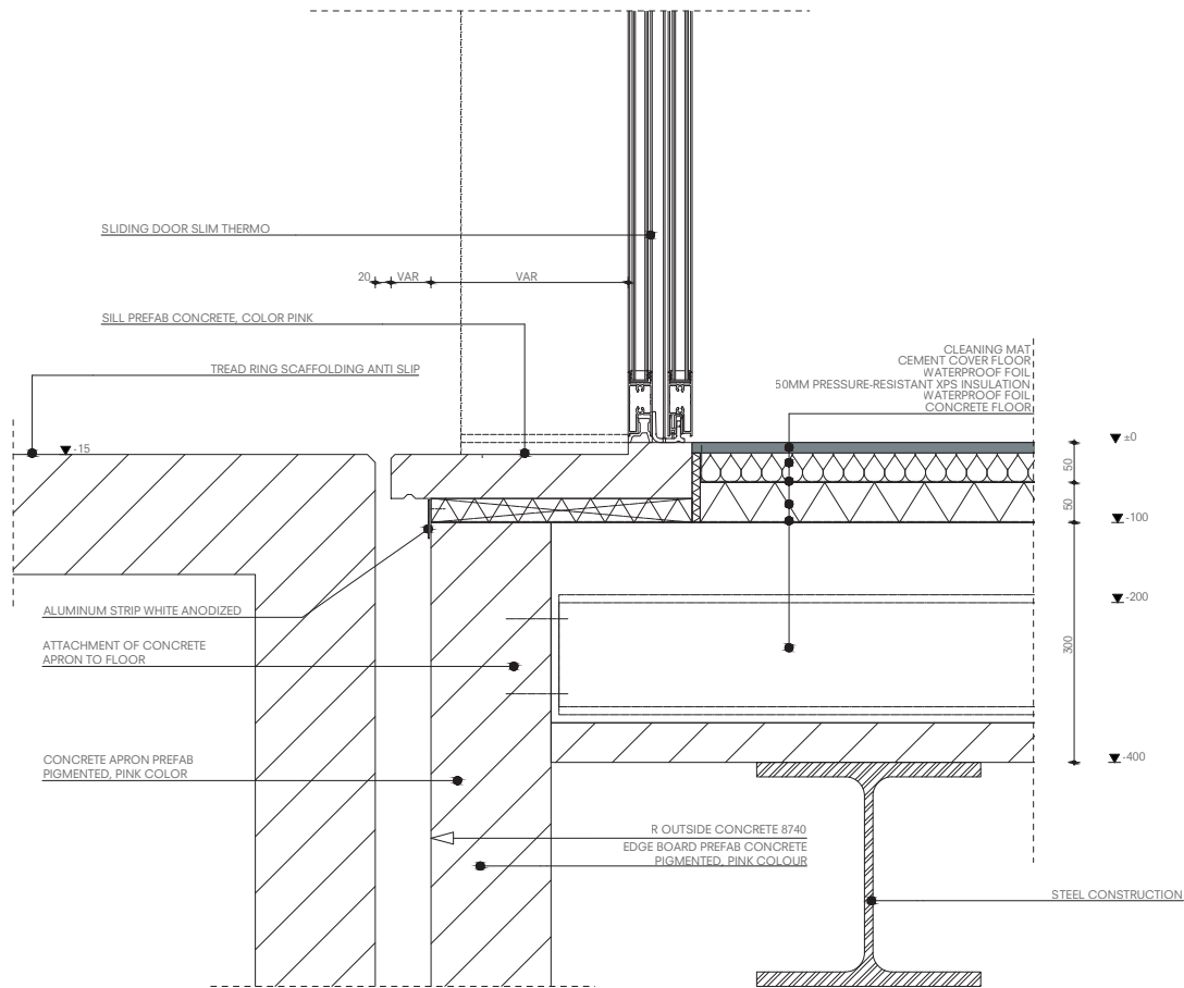
Detail 1: Platform - Pavilion floor connection
