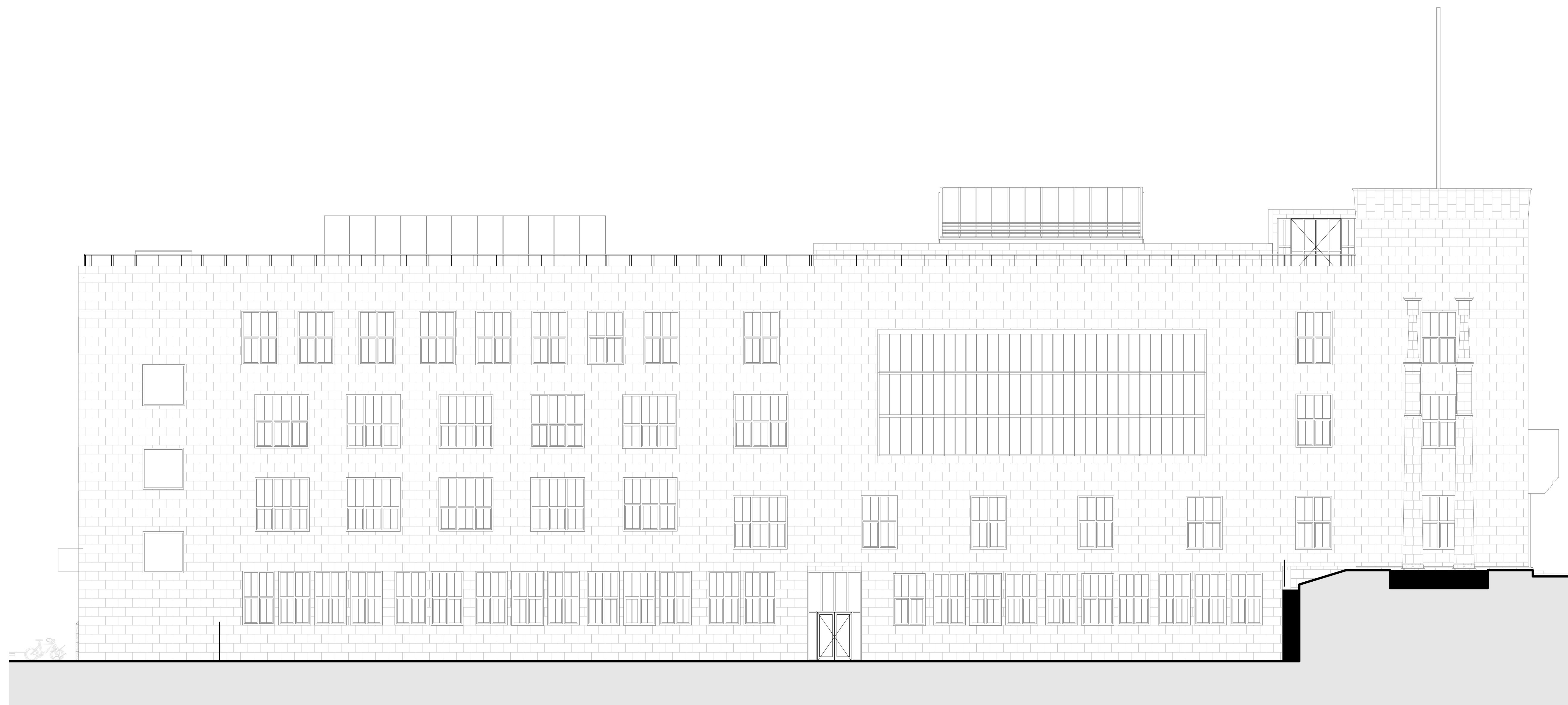
Elevation - West
