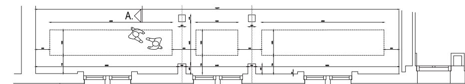
Plattegrond | verdieping 4 Floorplan | 4th floor
