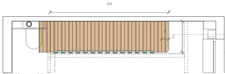
PLAN trap .01
