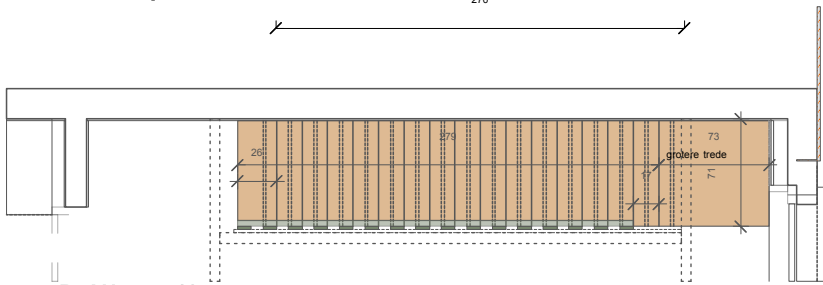
PLAN trap .12
