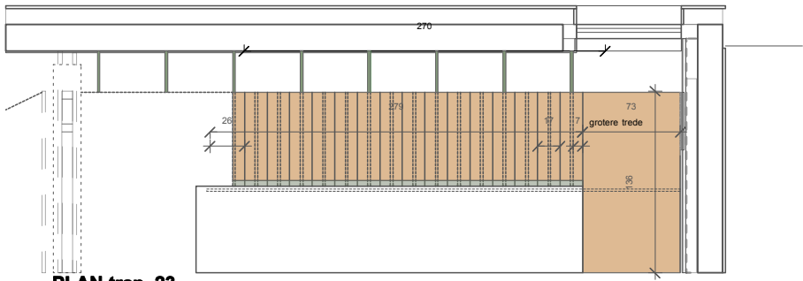
PLAN trap .23
