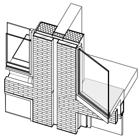
detail 371-308
