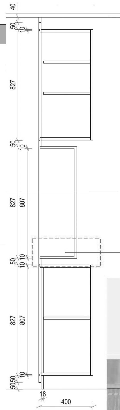
Detail Section A
