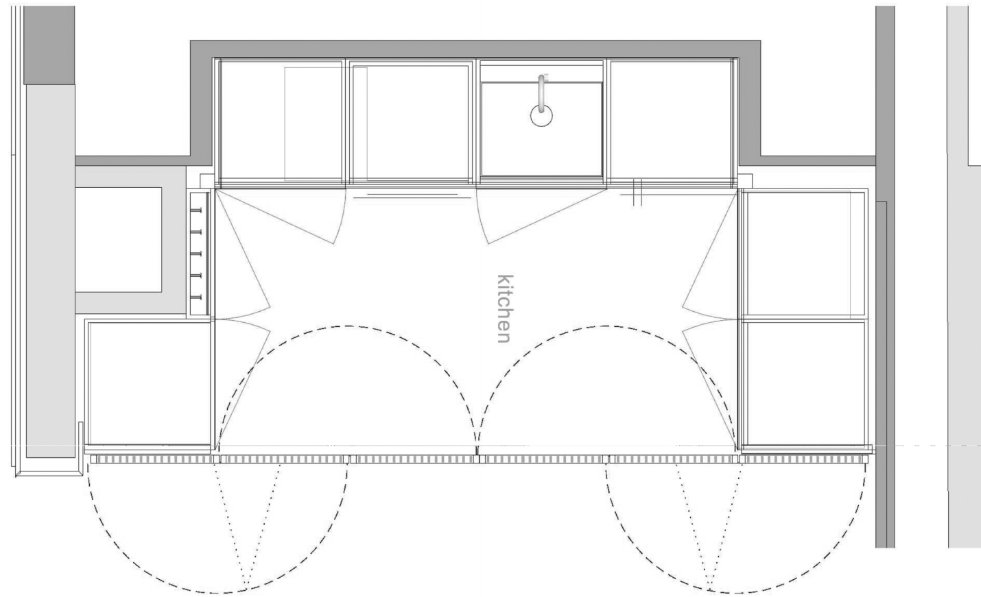
Top view - Door panels - open
