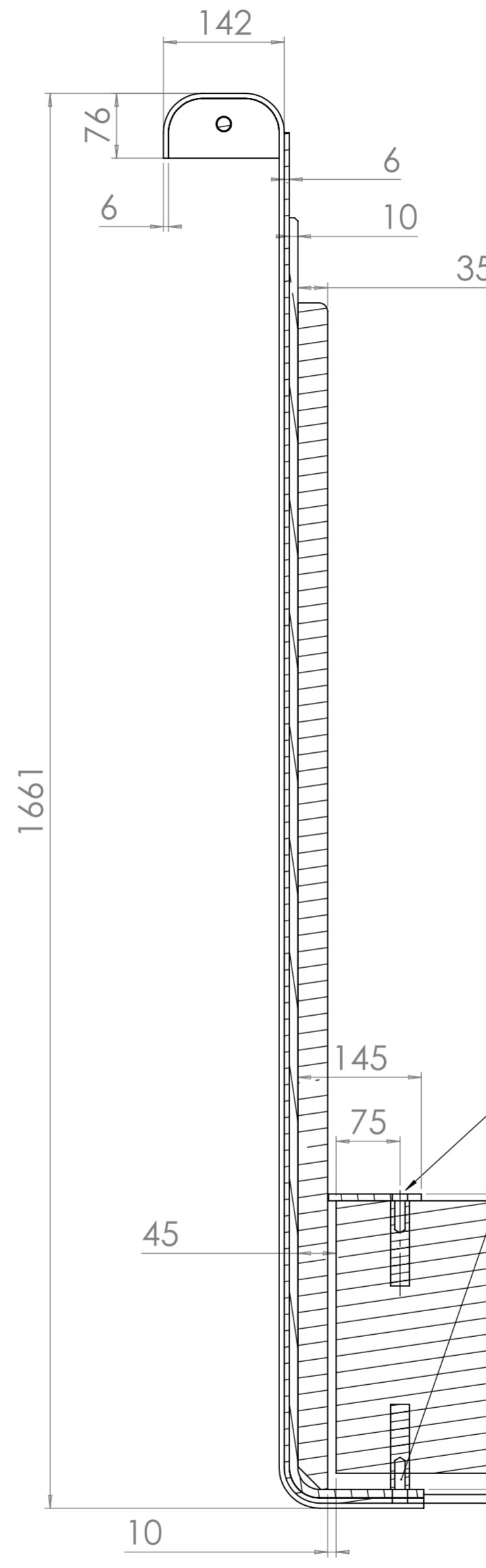
SECTION H-H
