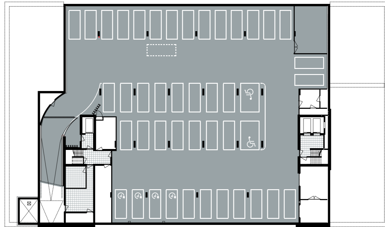
Garage kelder 1:175
