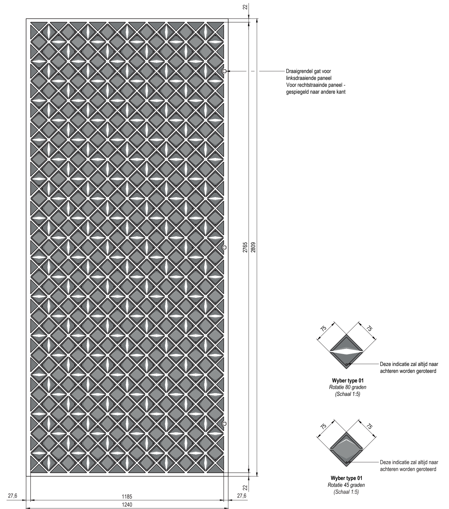
detail - panels
