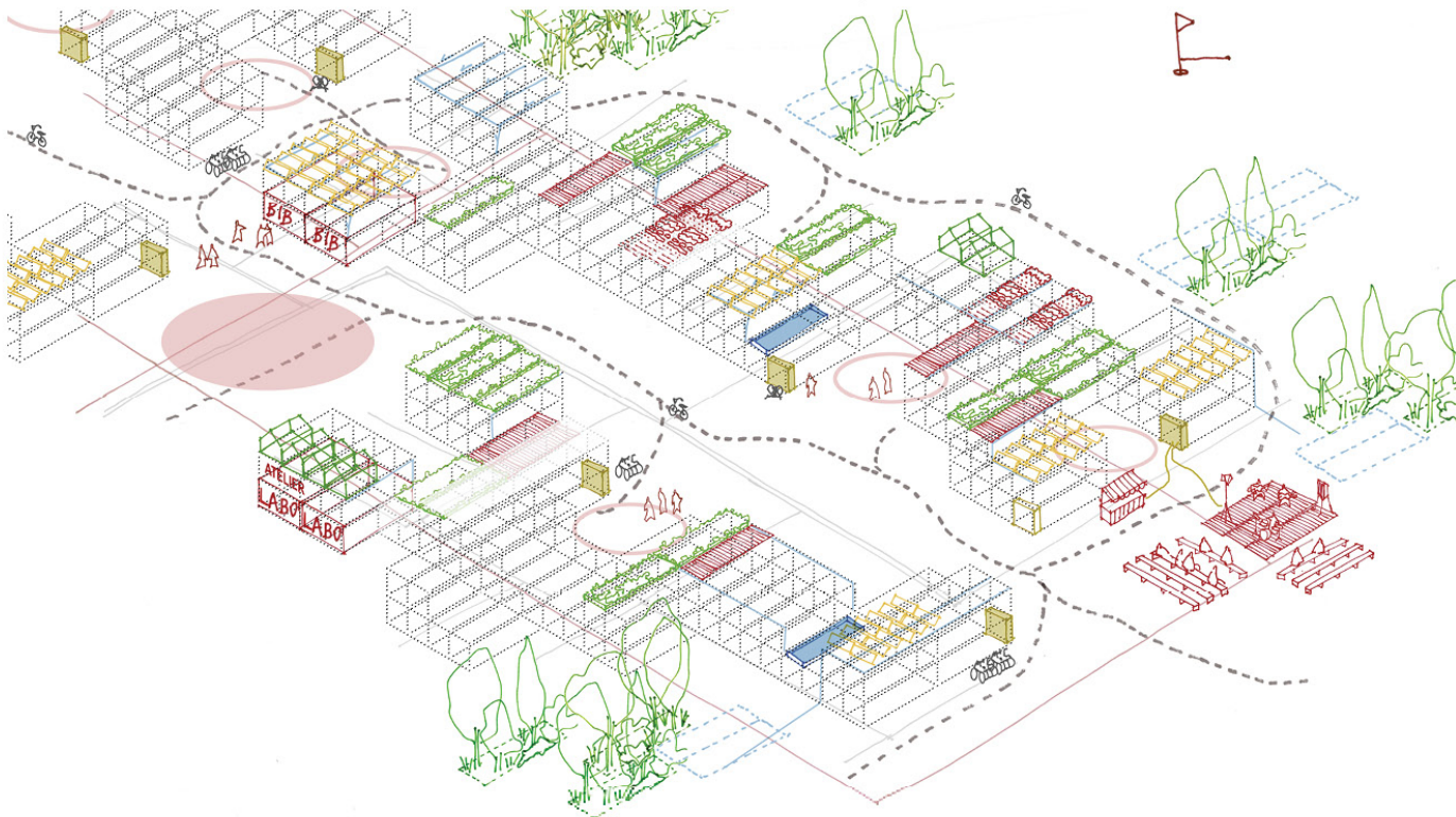
urban ecosystem
