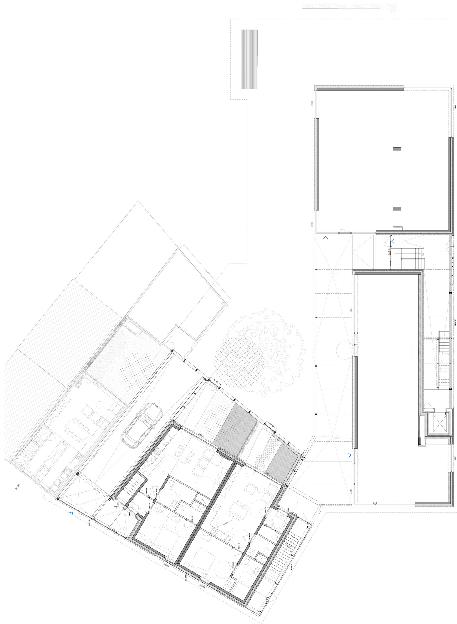
groundfloor plan apartments
