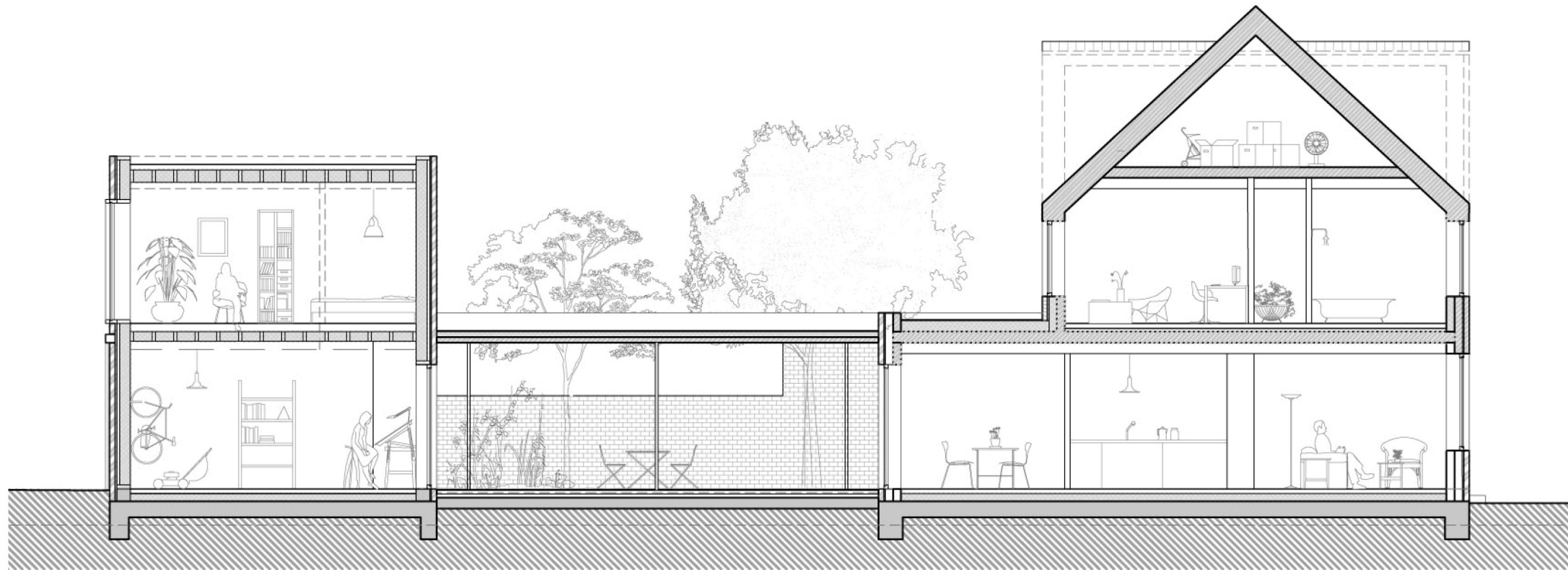
section corner house
