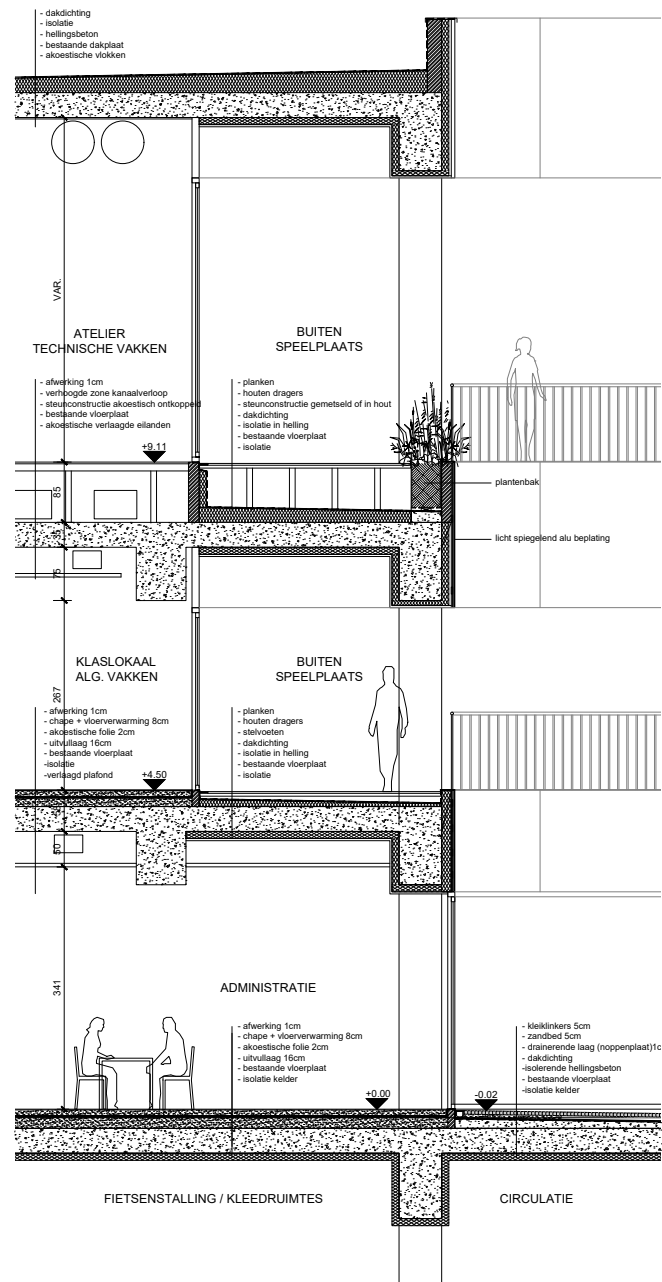
Vertical section detail of the new cut-out in the existing building with a raised floor on level +2 for technical ducts
